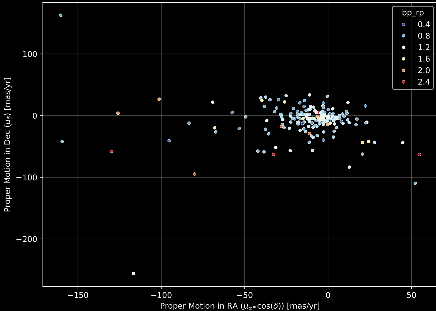
APOGEE DR17 Field: [018+46_MGA] Proper Motion Diagram (n= 191)
