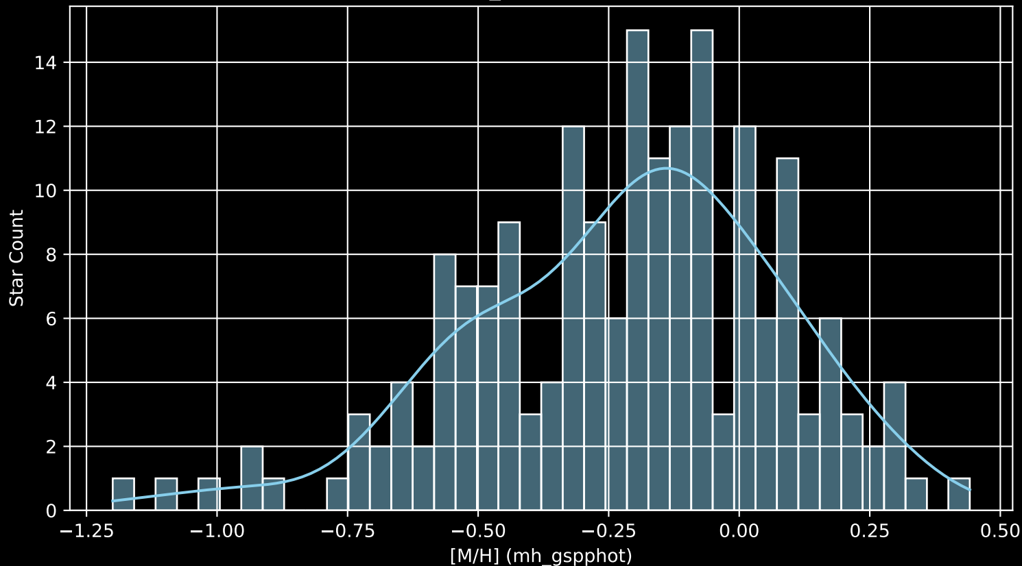
APOGEE DR17 Field: [018+46_MGA [M/H] (mh_gspphot) (n= 188)
