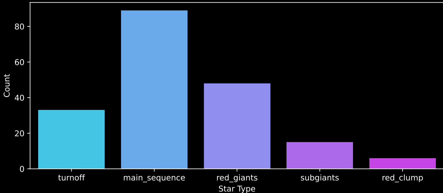
APOGEE DR17 Field: [018+46_MGA] Count plot of Star Type
