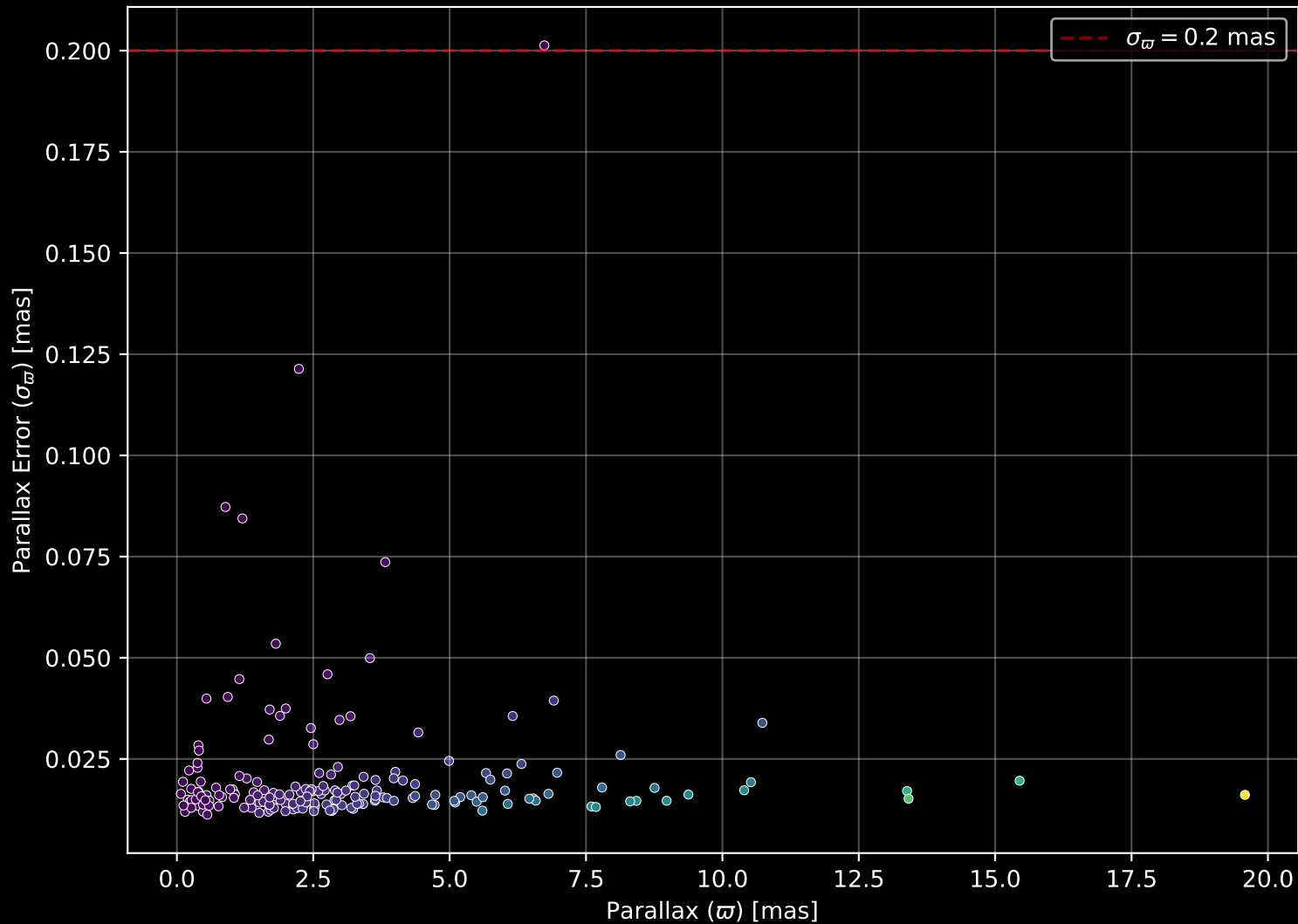
APOGEE DR17 Field: [018+46_MGA] Parallax Quality (n= 191)
