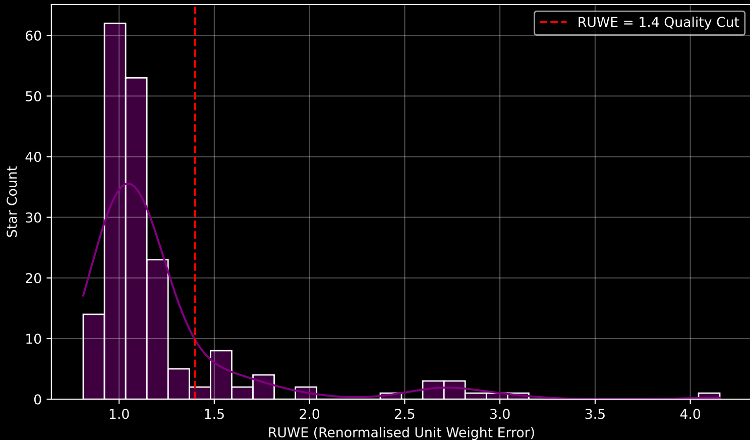
GAPOGEE DR17 Field [018+46_MGA] RUWE Distribution (n= 186)
