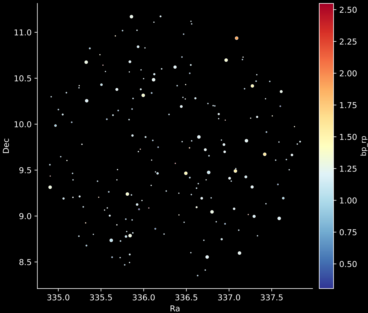
APOGEE DR17 Field: [018+46_MGA] Stars: 191
