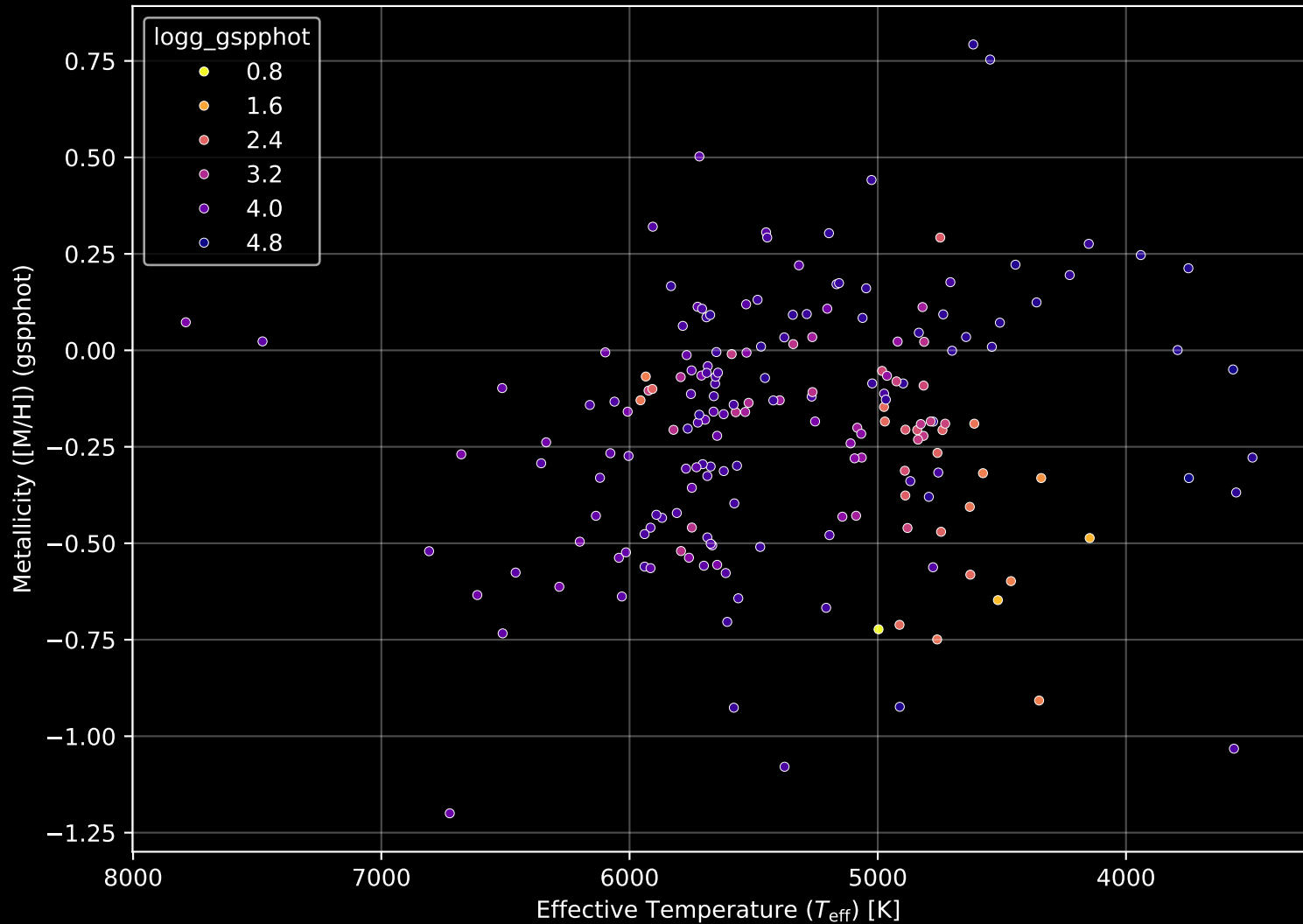
APOGEE DR17 Field: [018+46_MGA] Stellar Population Parameters (n= 191)
